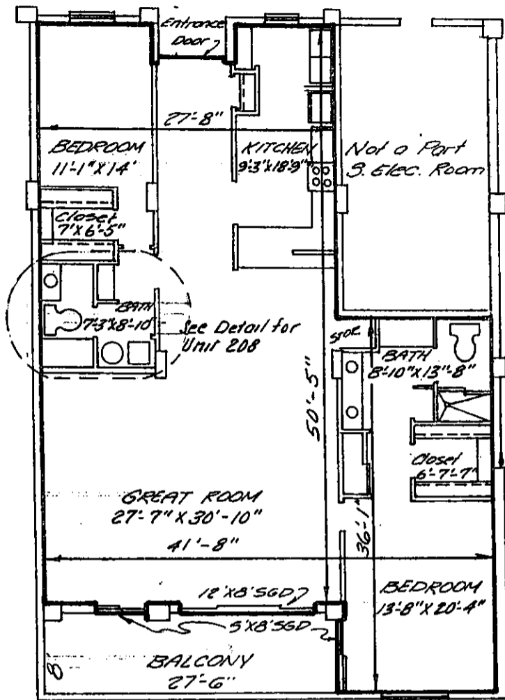
TYPICAL UNIT "1D"
