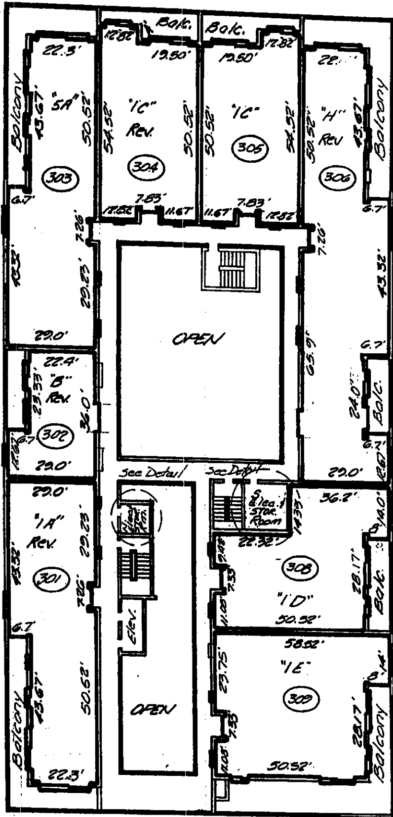
3rd. FLOOR PLAN
