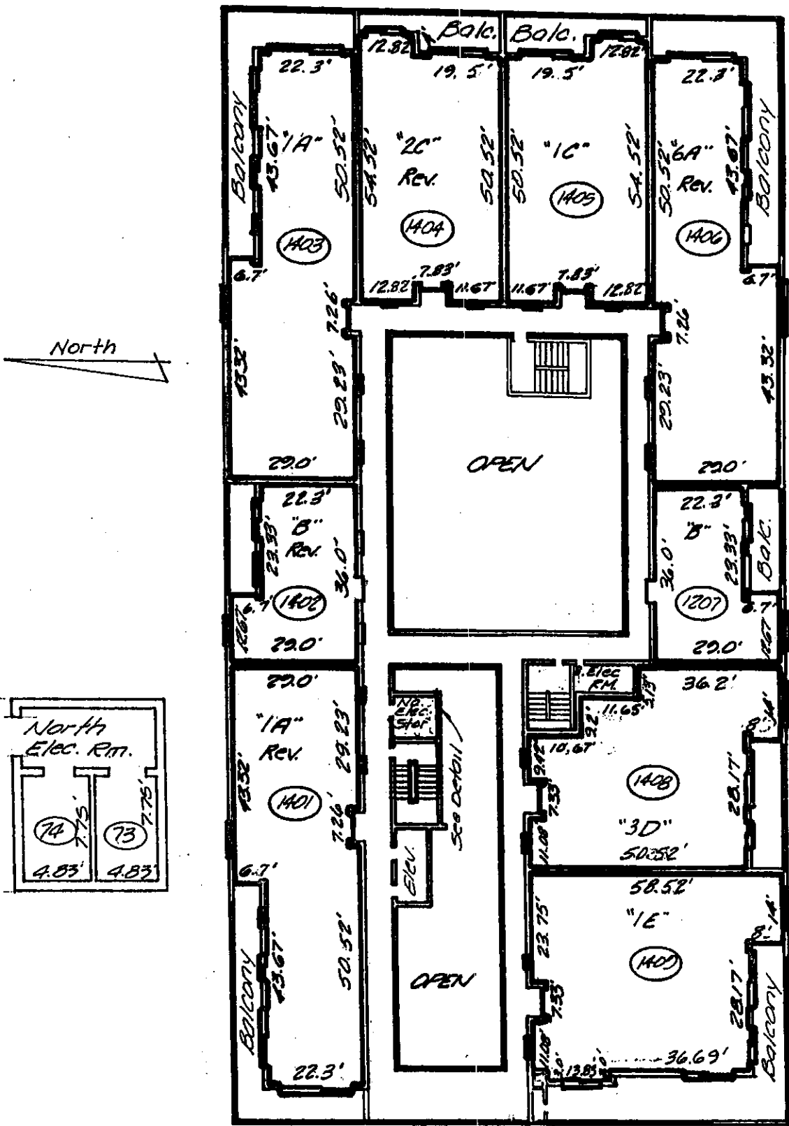
14th. FLOOR PLAN
