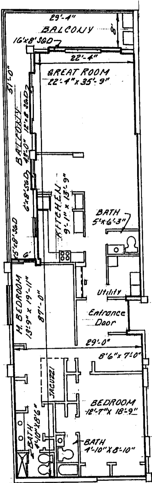
TYPICAL UNIT "3A"
