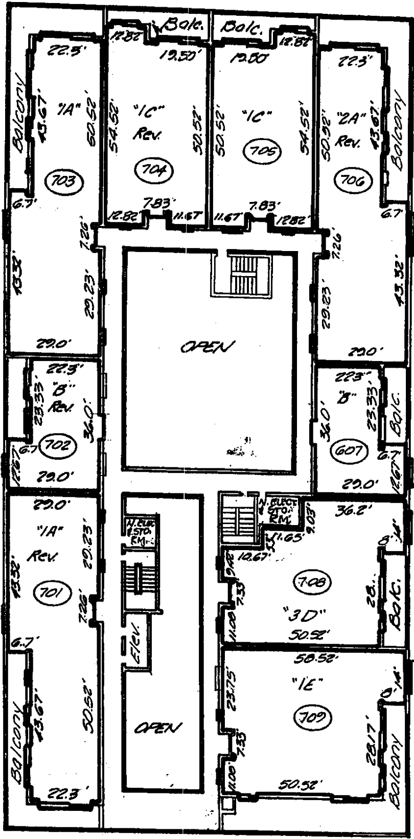
7th. FLOOR PLAN
